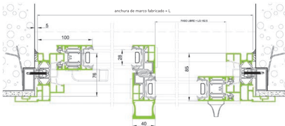
Corredera 2 railes
