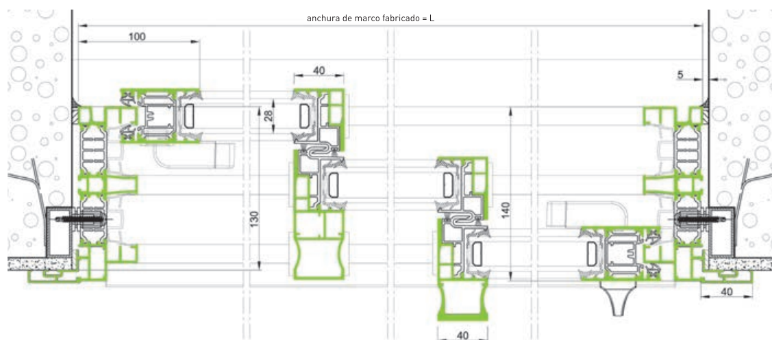
Corredera 3 railes
